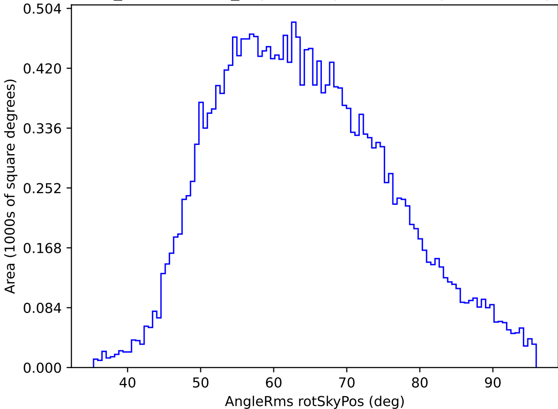
weather_cloudso0v3.4_10yrs All sky u band: AngleRms rotSkyPos
