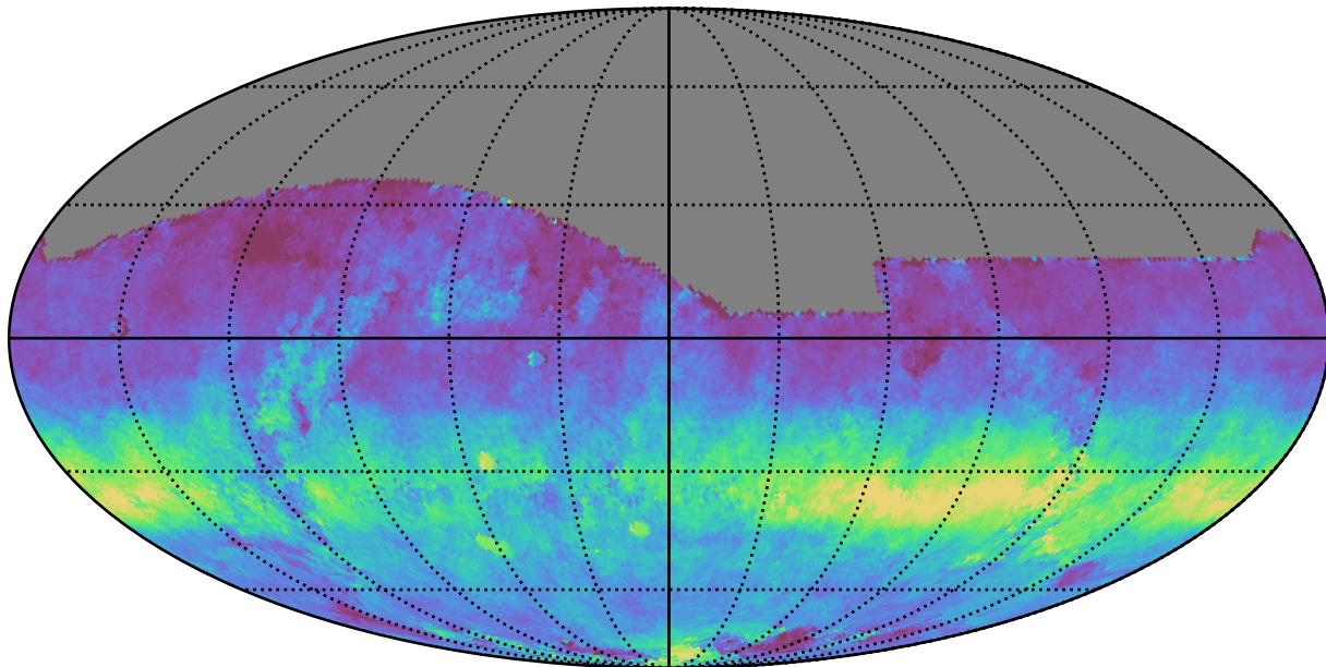
weather_cloudso0v3.4_10yrs All sky r band: AngleRms rotSkyPos
