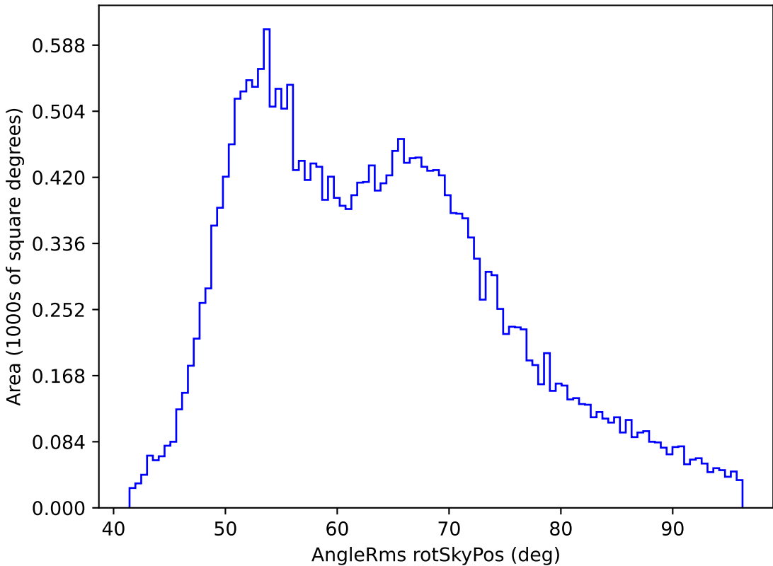
weather_cloudso0v3.4_10yrs All sky r band: AngleRms rotSkyPos
