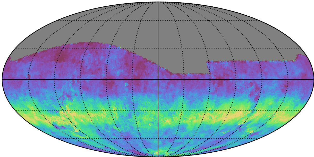
weather_cloudso0v3.4_10yrs All sky g band: AngleRms rotSkyPos
