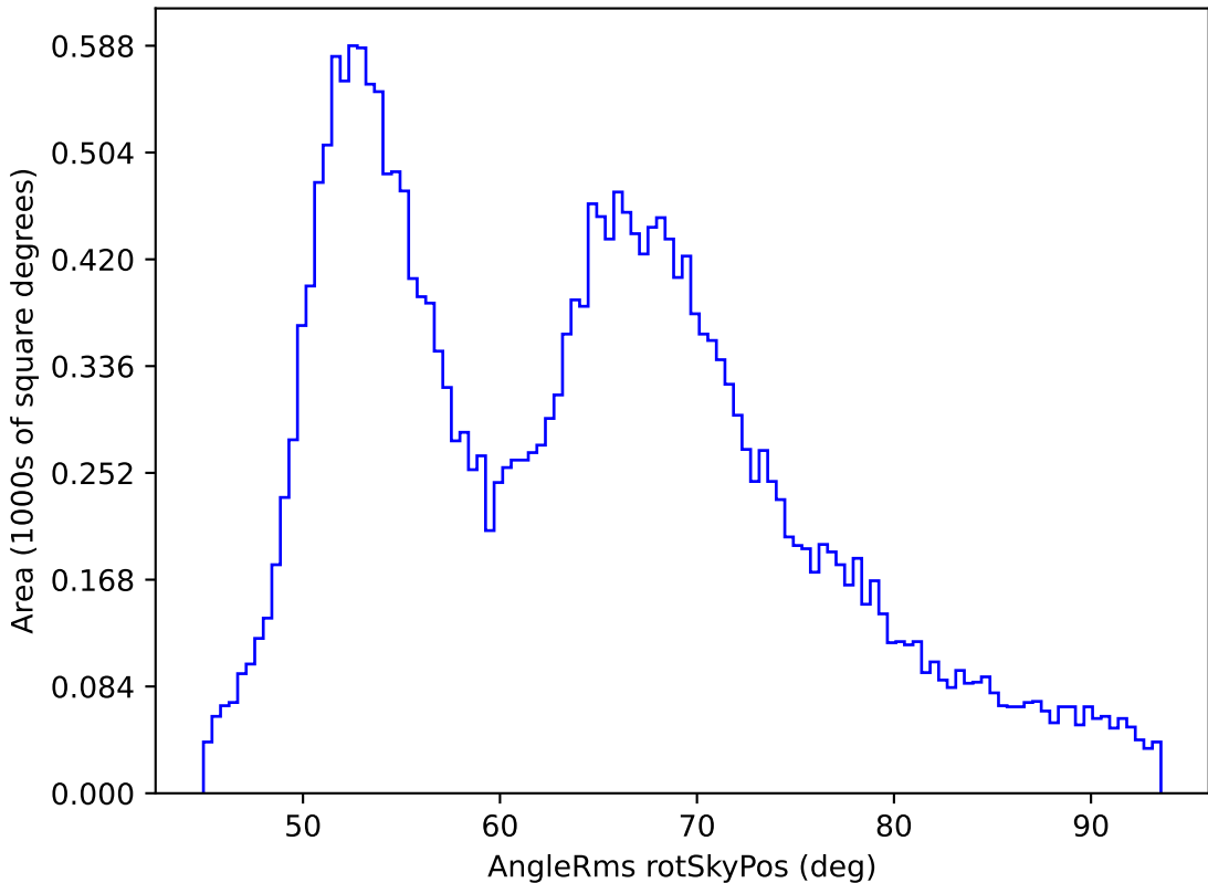
weather_cloudso0v3.4_10yrs All sky all bands: AngleRms rotSkyPos
