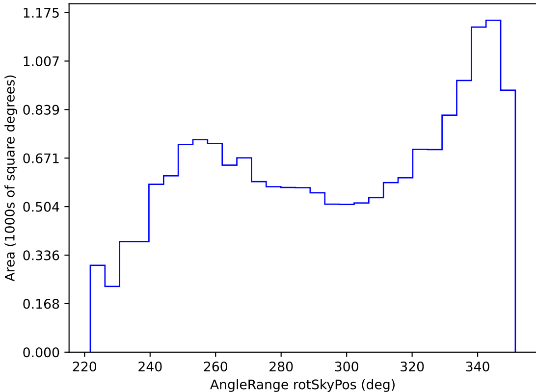
weather_cloudso0v3.4_10yrs WFD all bands: AngleRange rotSkyPos
