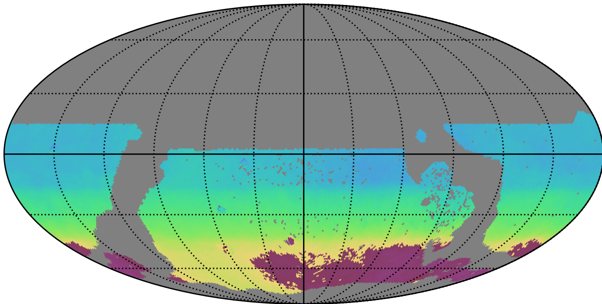
weather_cloudso0v3.4_10yrs WFD all bands: AngleMean rotSkyPos
