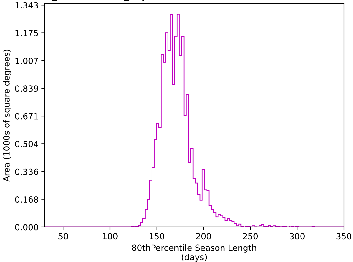
weather_cloudso0v3.4_10yrs WFD z band: 80thPercentile Season Length
