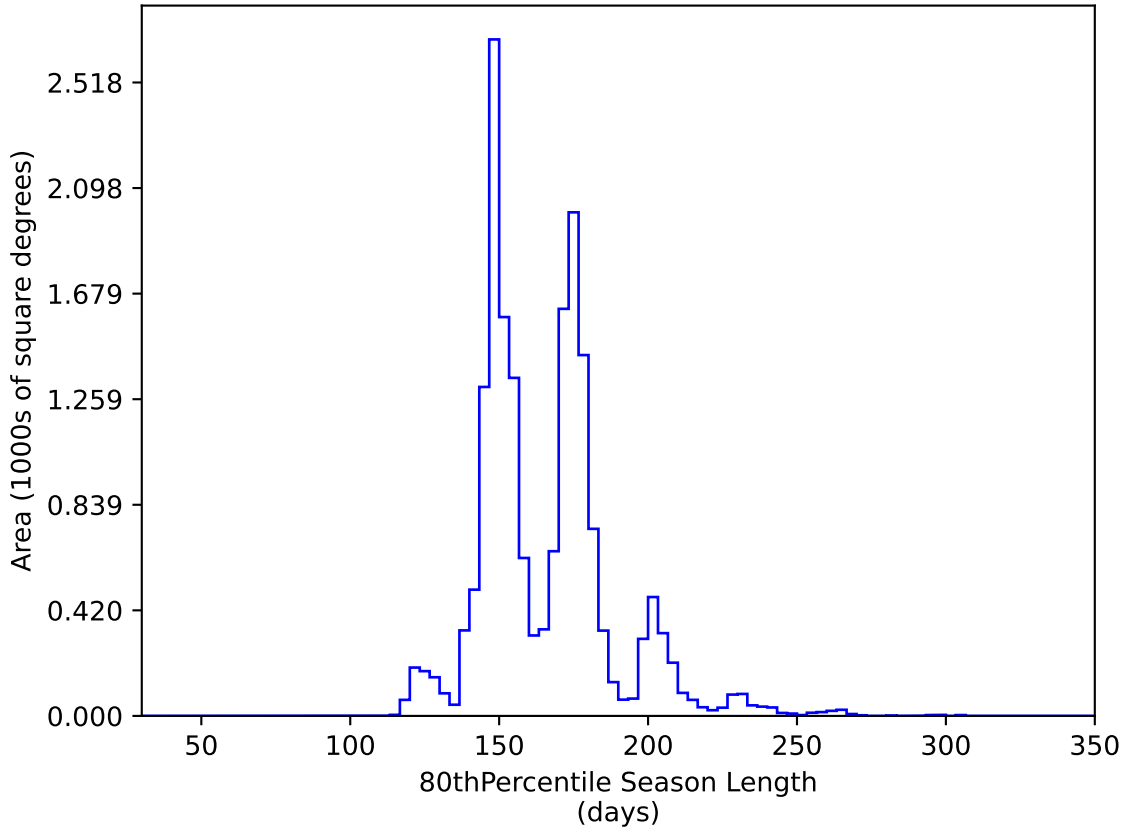
weather_cloudso0v3.4_10yrs WFD y band: 80thPercentile Season Length
