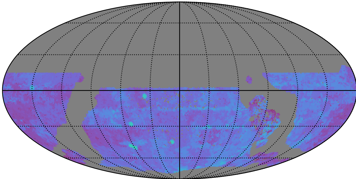
weather_cloudso0v3.4_10yrs WFD u band: 80thPercentile Season Length
