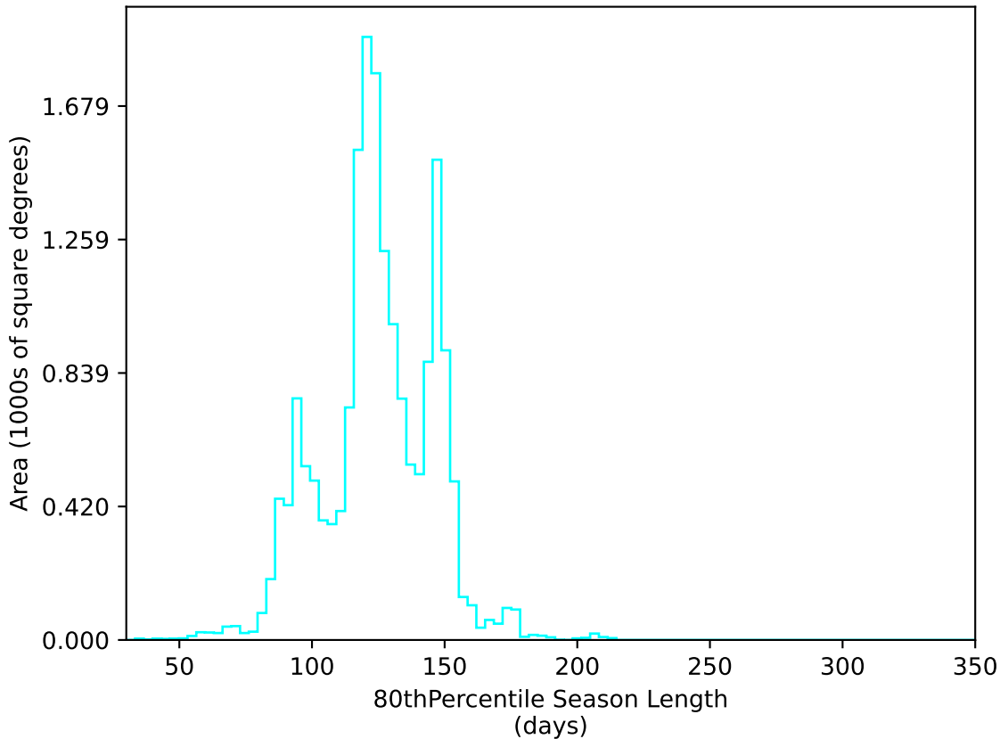
weather_cloudso0v3.4_10yrs WFD u band: 80thPercentile Season Length
