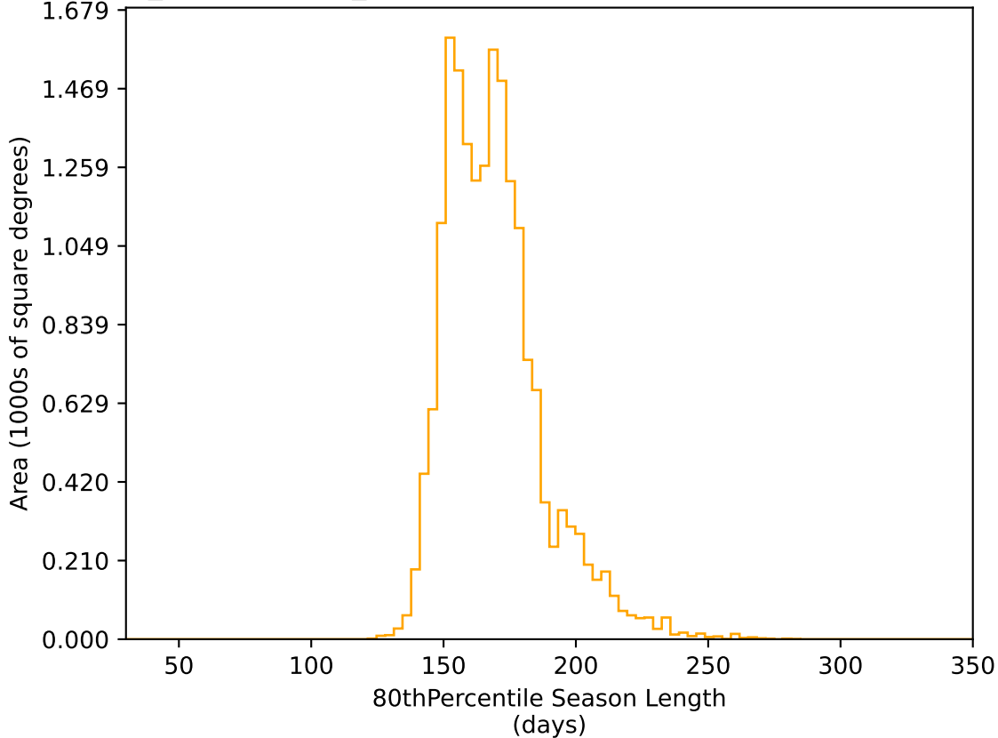
weather_cloudso0v3.4_10yrs WFD r band: 80thPercentile Season Length
