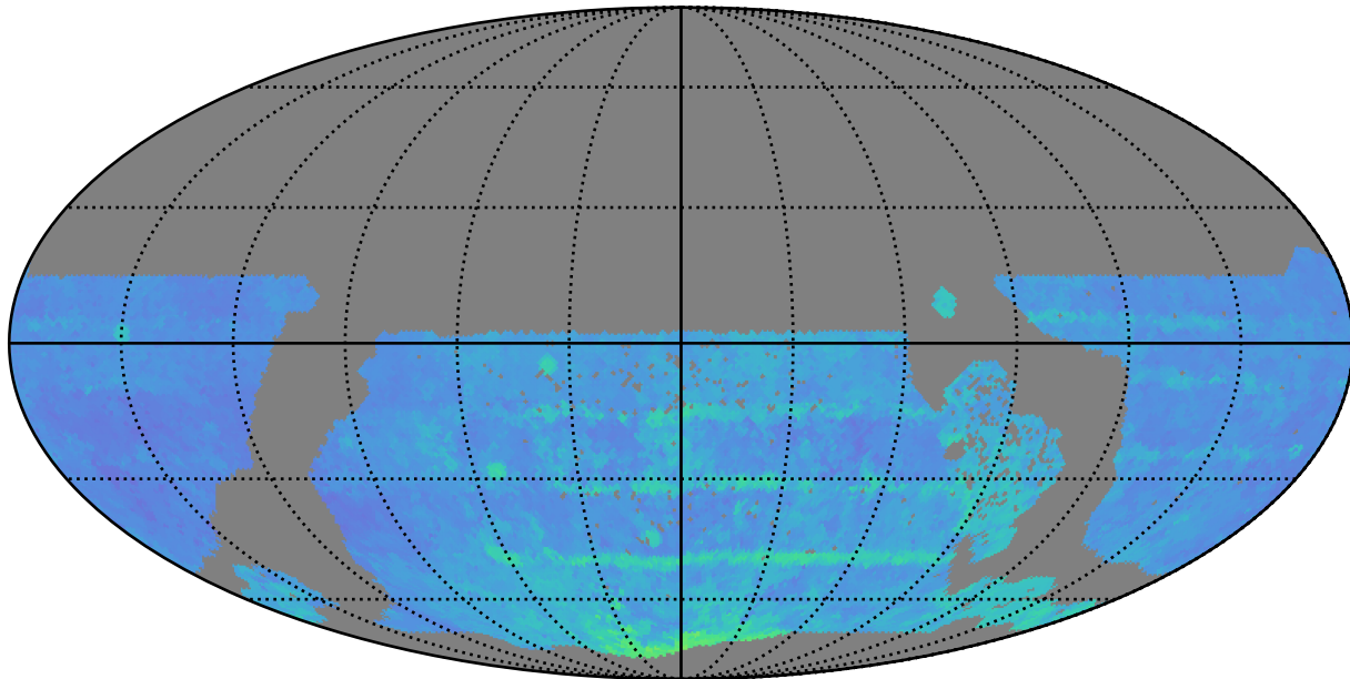
weather_cloudso0v3.4_10yrs WFD i band: 80thPercentile Season Length
