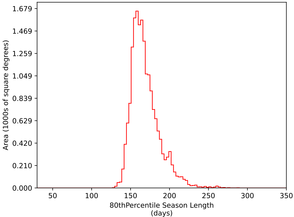
weather_cloudso0v3.4_10yrs WFD i band: 80thPercentile Season Length
