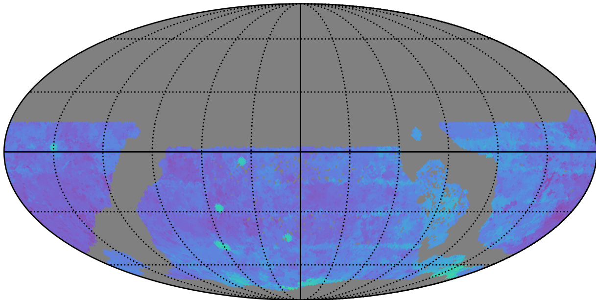
weather_cloudso0v3.4_10yrs WFD g band: 80thPercentile Season Length
