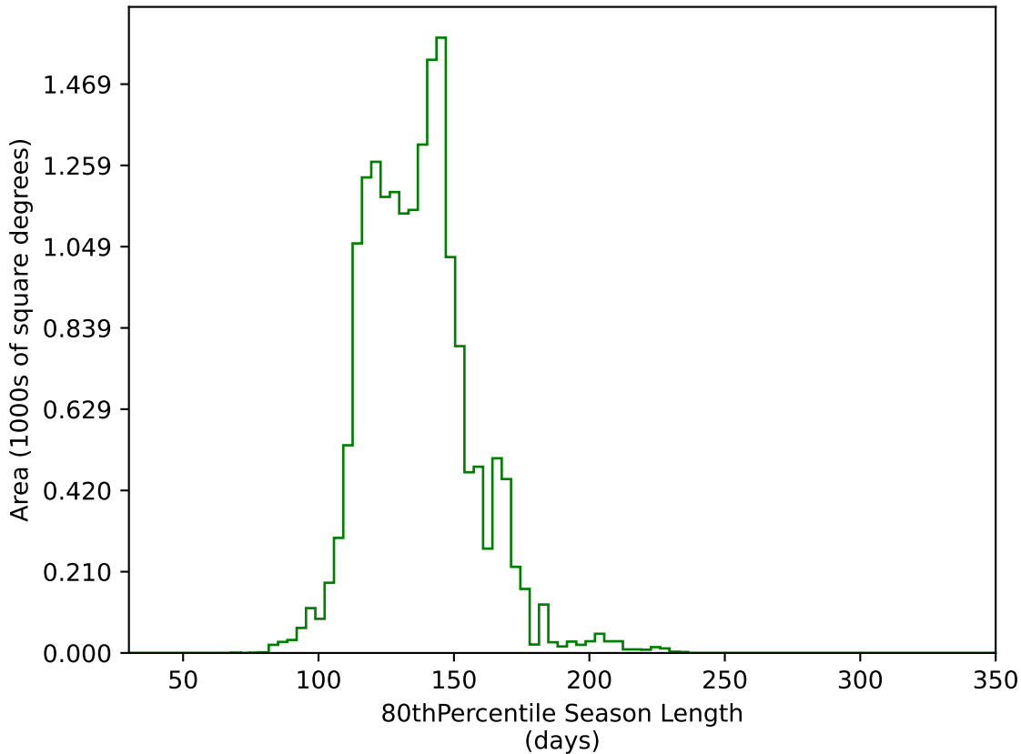
weather_cloudso0v3.4_10yrs WFD g band: 80thPercentile Season Length
