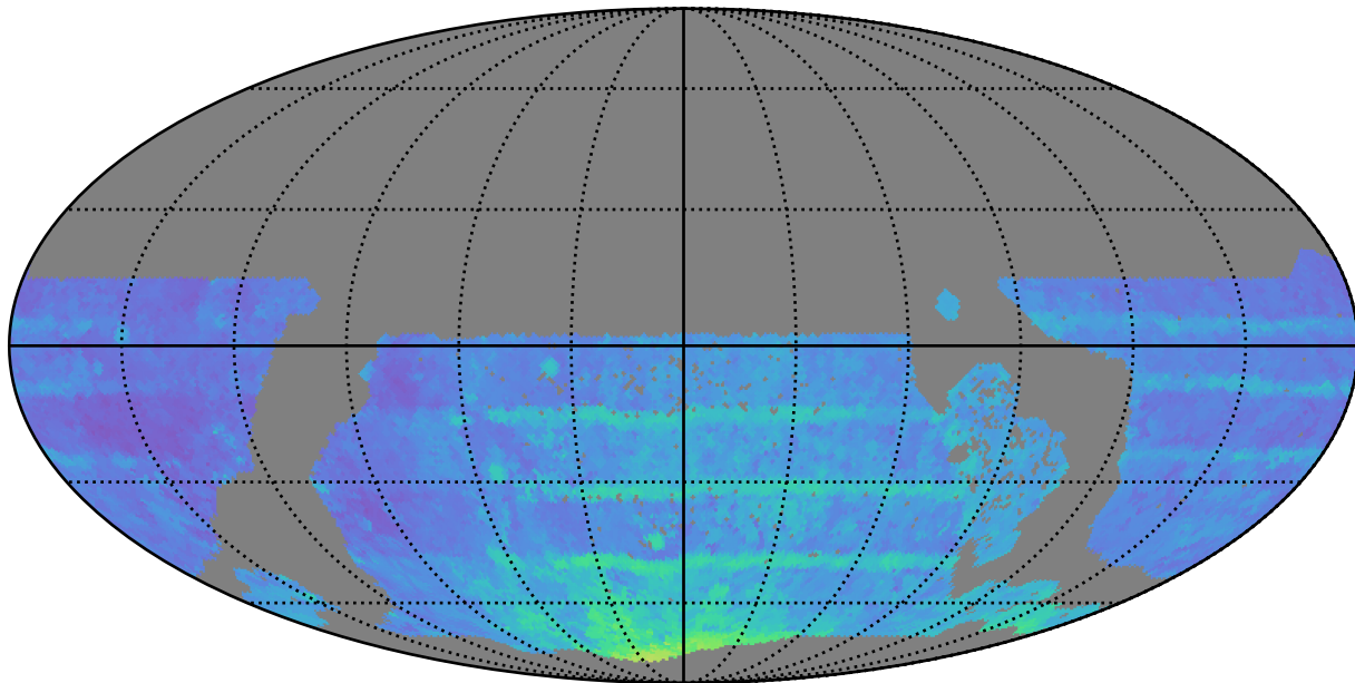
weather_cloudso0v3.4_10yrs WFD all bands: 80thPercentile Season Length
