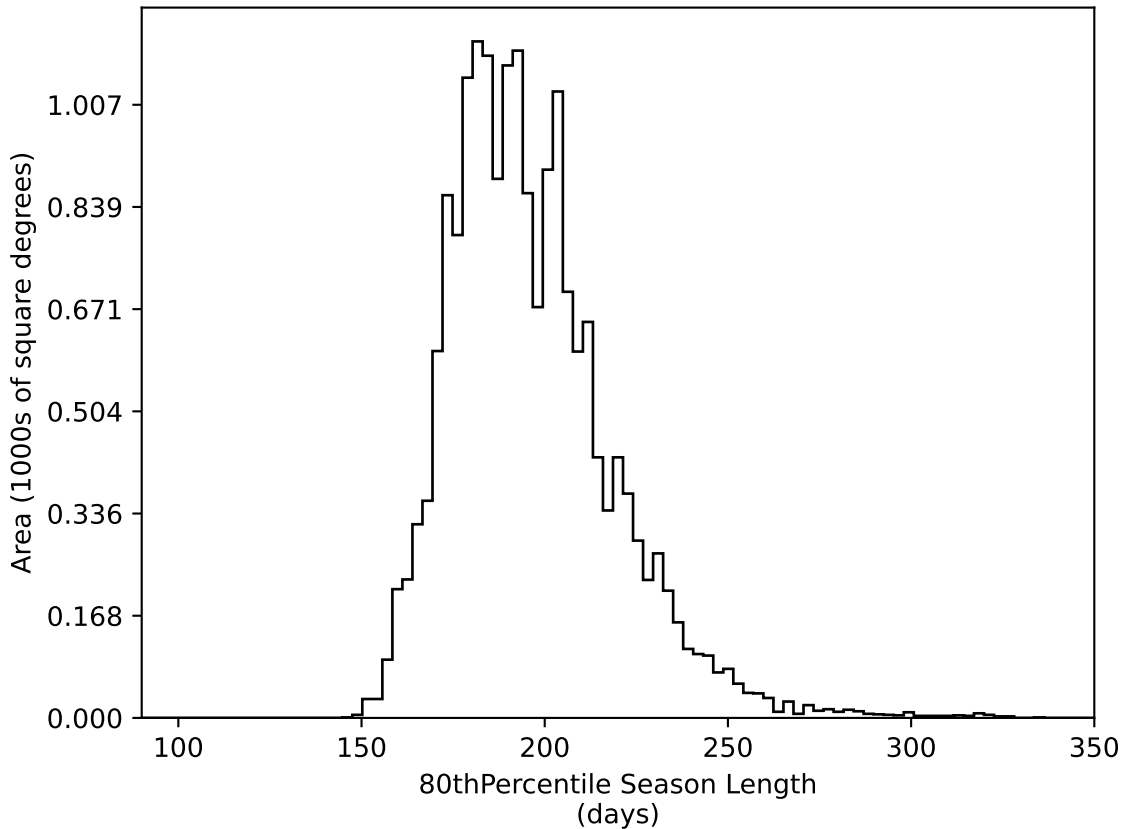
weather_cloudso0v3.4_10yrs WFD all bands: 80thPercentile Season Length
