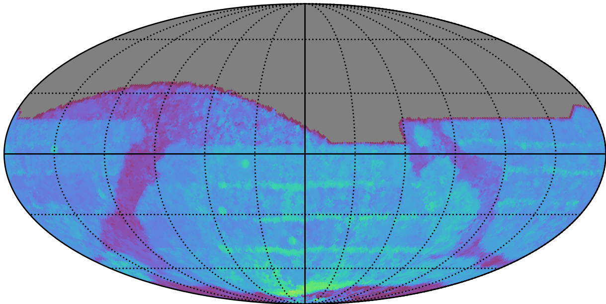
weather_cloudso0v3.4_10yrs All sky z band: 80thPercentile Season Length
