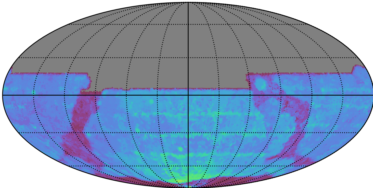
weather_cloudso0v3.4_10yrs All sky y band: 80thPercentile Season Length
