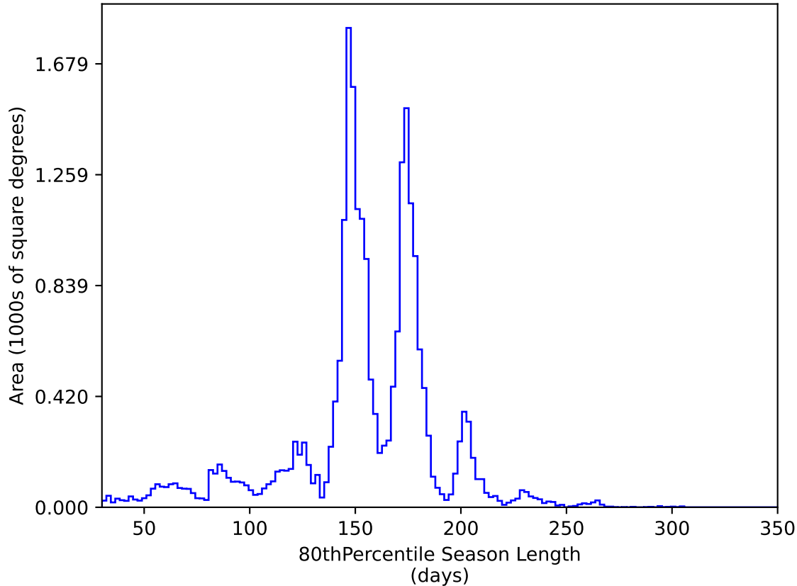
weather_cloudso0v3.4_10yrs All sky y band: 80thPercentile Season Length
