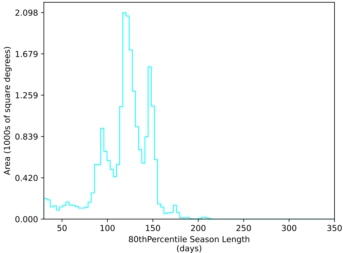
weather_cloudso0v3.4_10yrs All sky u band: 80thPercentile Season Length
