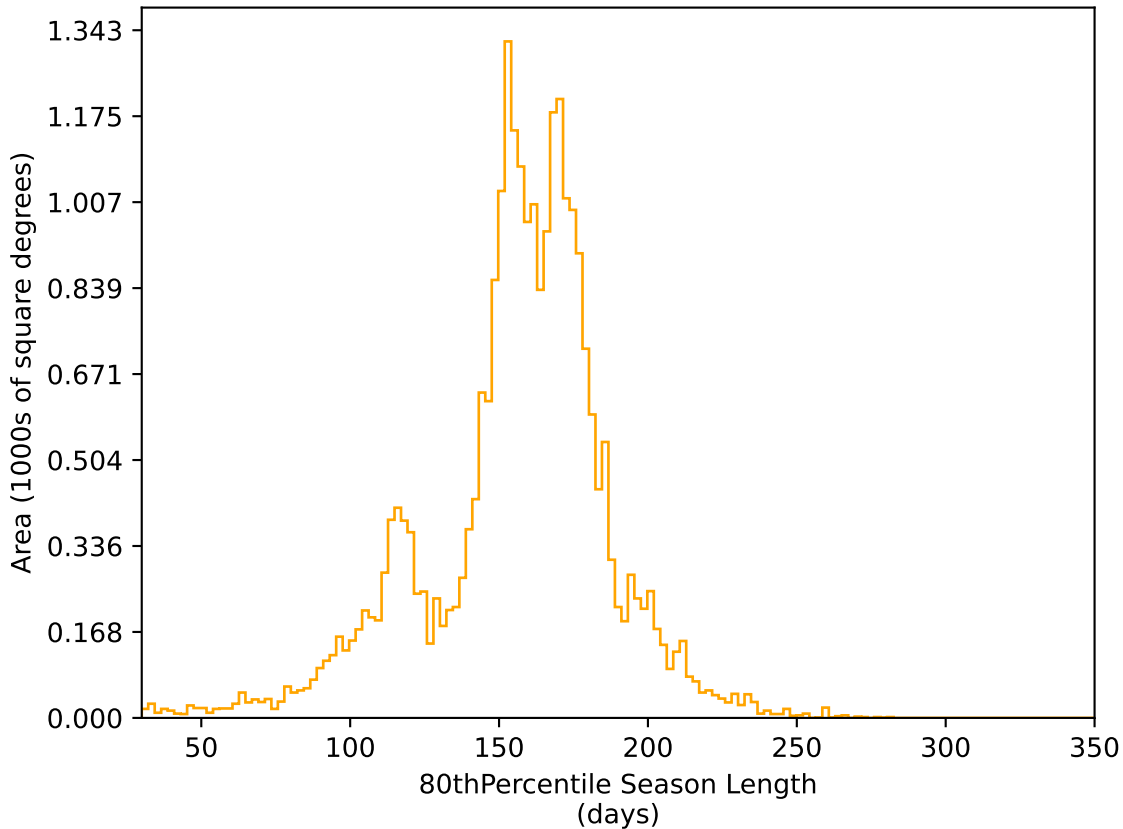
weather_cloudso0v3.4_10yrs All sky r band: 80thPercentile Season Length
