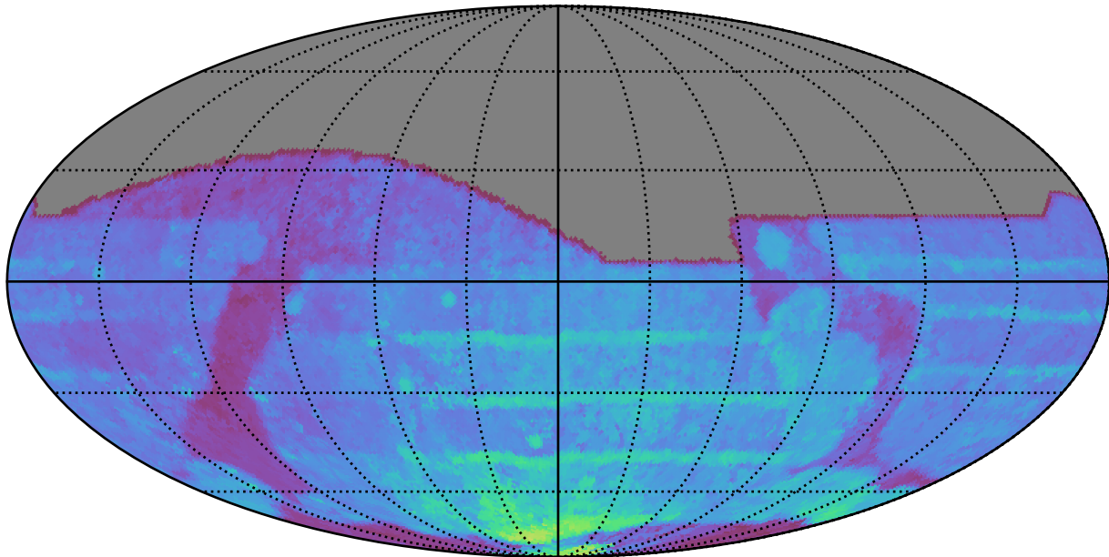
weather_cloudso0v3.4_10yrs All sky all bands: 80thPercentile Season Length
