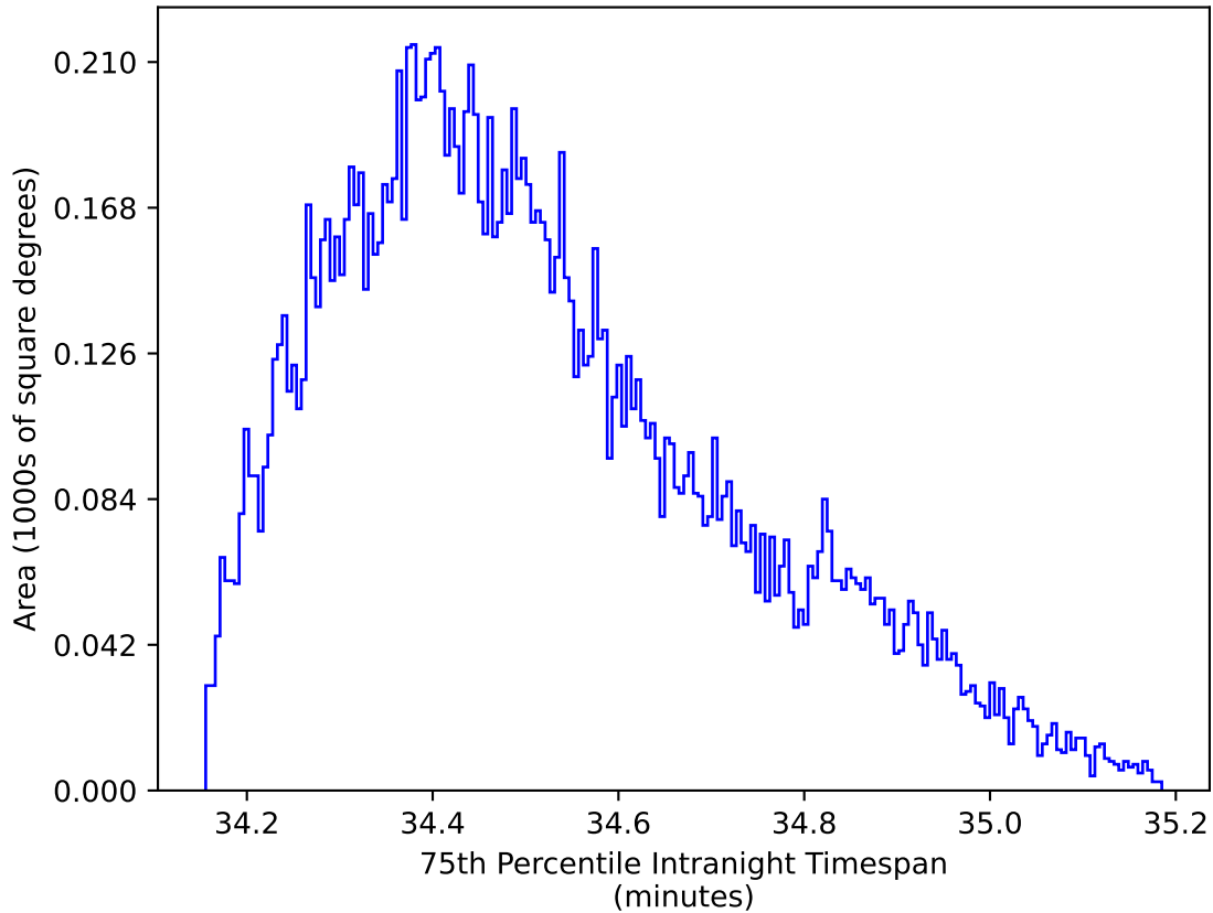
weather_cloudso0v3.4_10yrs WFD zy bands: 75th Percentile Intranight Timespan
