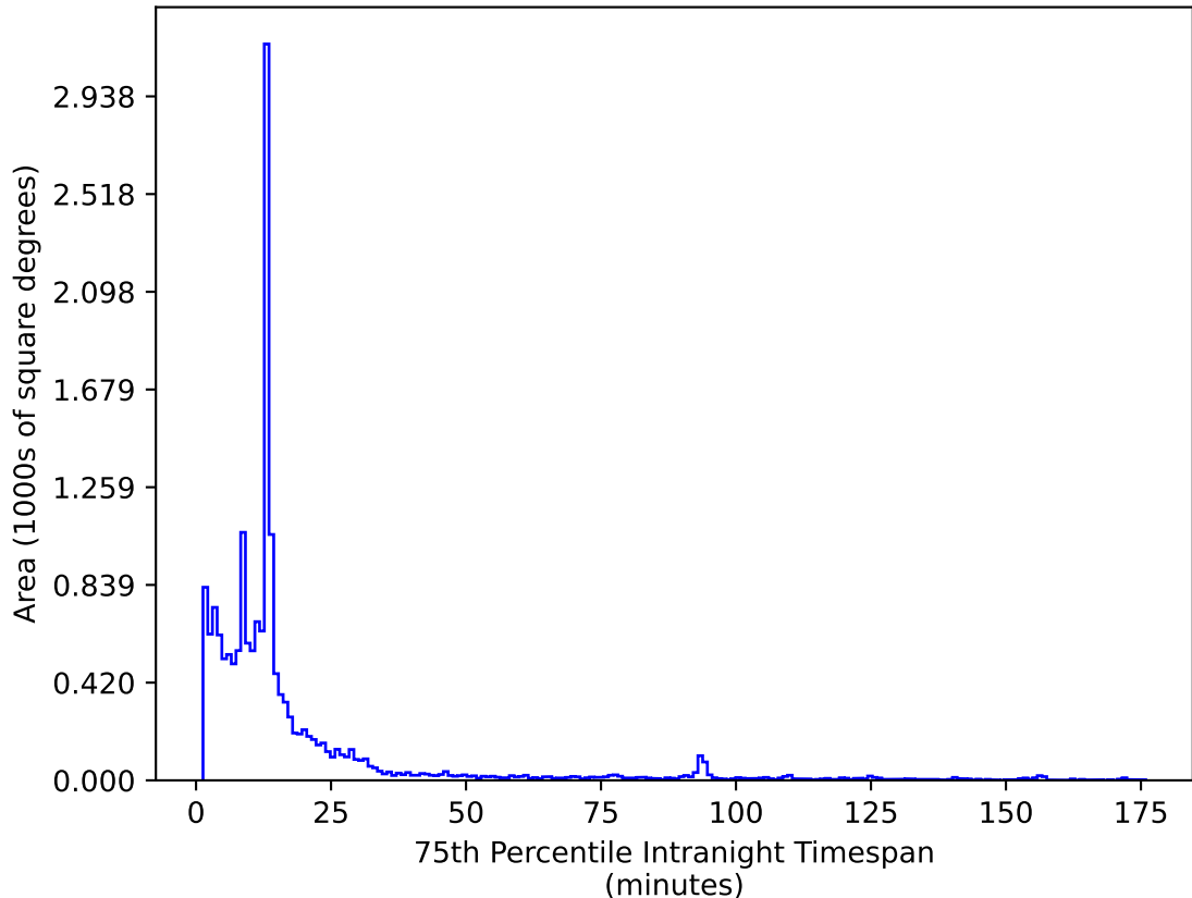
weather_cloudso0v3.4_10yrs WFD z band: 75th Percentile Intranight Timespan
