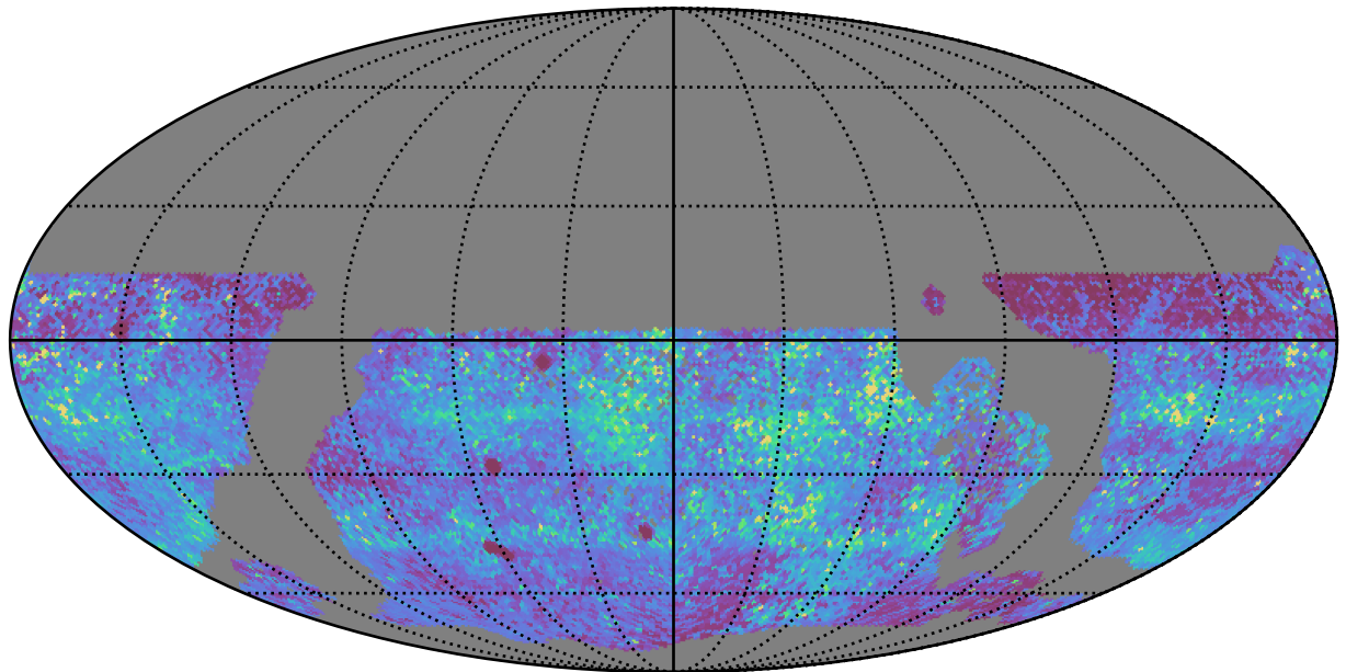
weather_cloudso0v3.4_10yrs WFD y band: 75th Percentile Intranight Timespan
