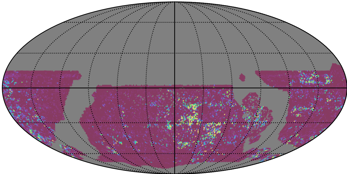
weather_cloudso0v3.4_10yrs WFD u band: 75th Percentile Intranight Timespan
