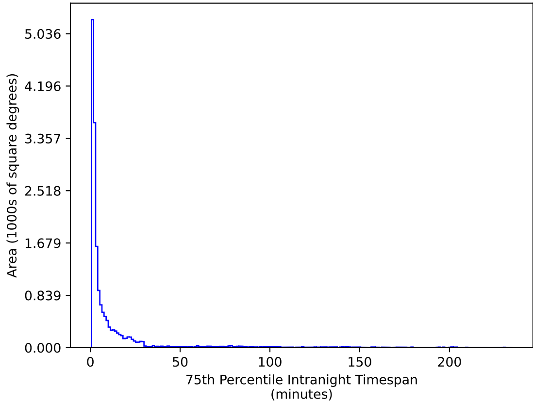
weather_cloudso0v3.4_10yrs WFD u band: 75th Percentile Intranight Timespan
