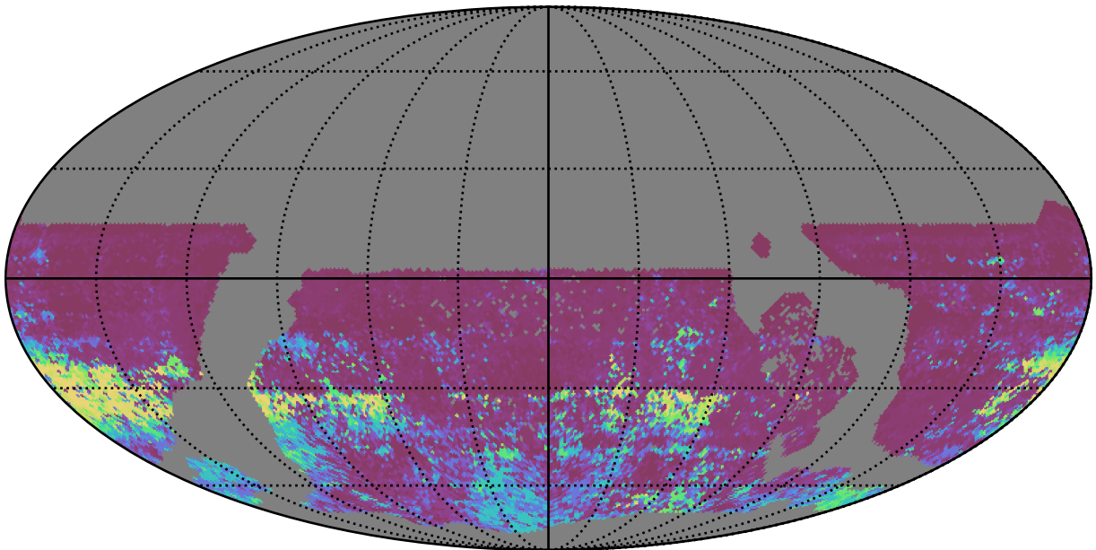
weather_cloudso0v3.4_10yrs WFD r band: 75th Percentile Intranight Timespan
