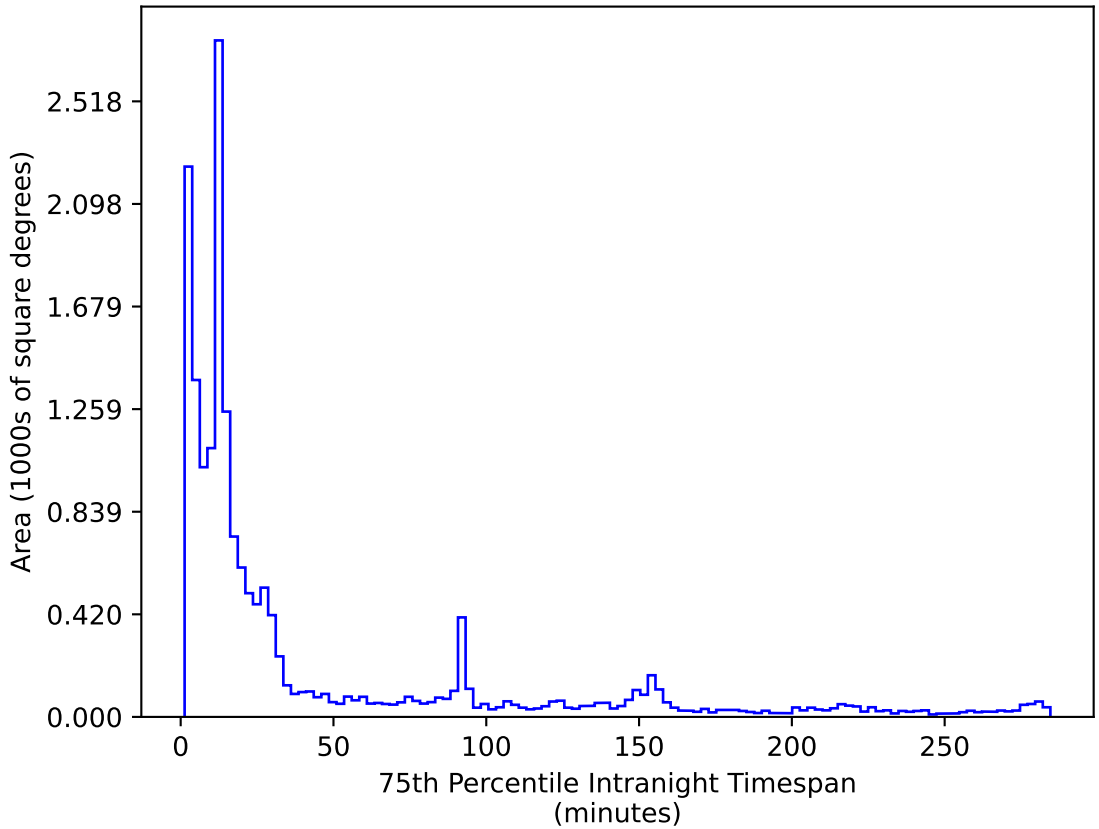
weather_cloudso0v3.4_10yrs WFD r band: 75th Percentile Intranight Timespan
