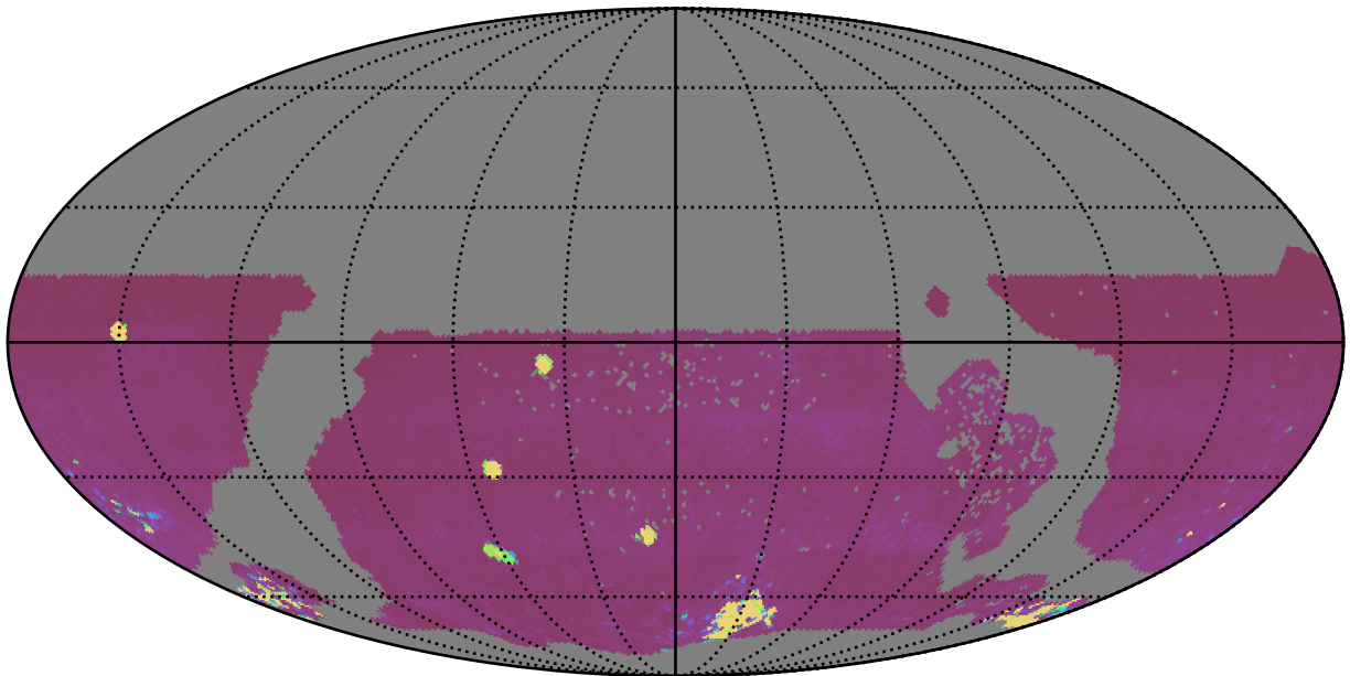
weather_cloudso0v3.4_10yrs WFD iz bands: 75th Percentile Intranight Timespan
