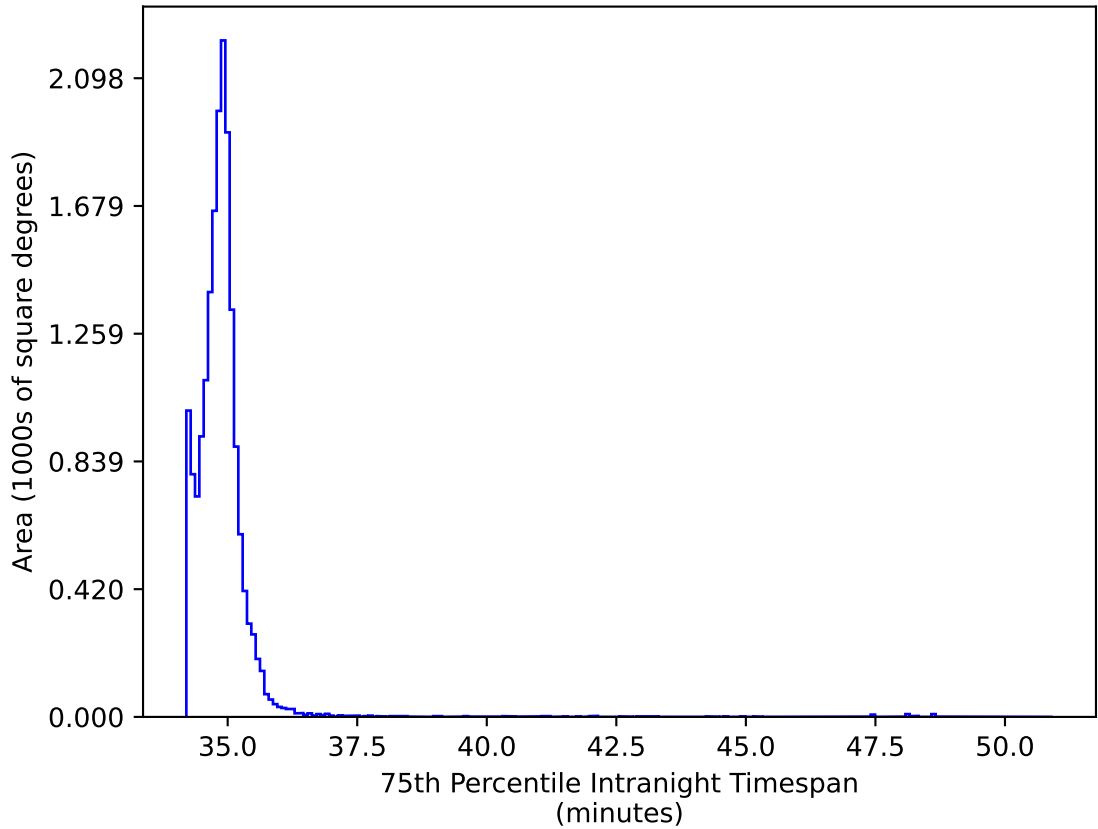
weather_cloudso0v3.4_10yrs WFD iz bands: 75th Percentile Intranight Timespan
