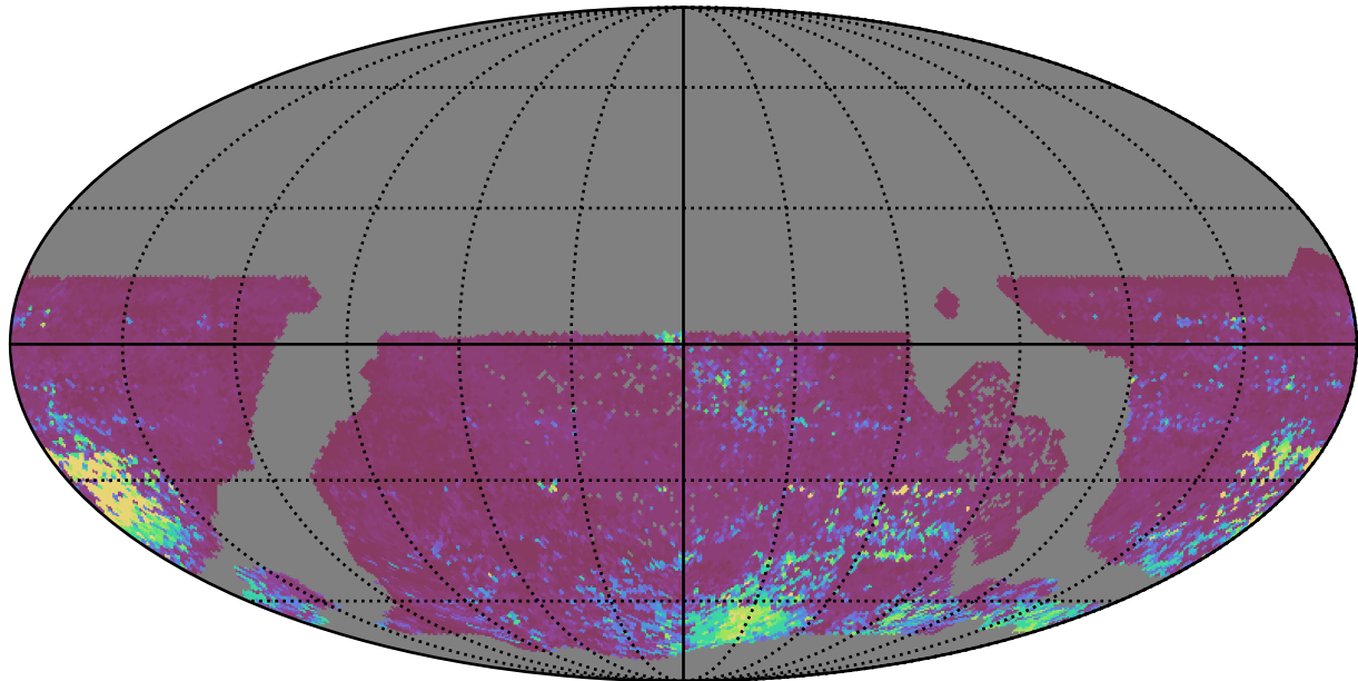
weather_cloudso0v3.4_10yrs WFD i band: 75th Percentile Intranight Timespan
