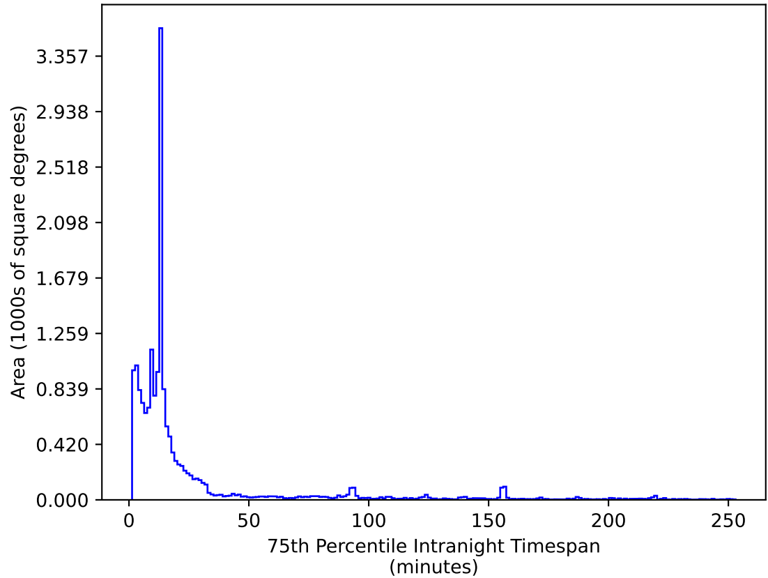
weather_cloudso0v3.4_10yrs WFD i band: 75th Percentile Intranight Timespan
