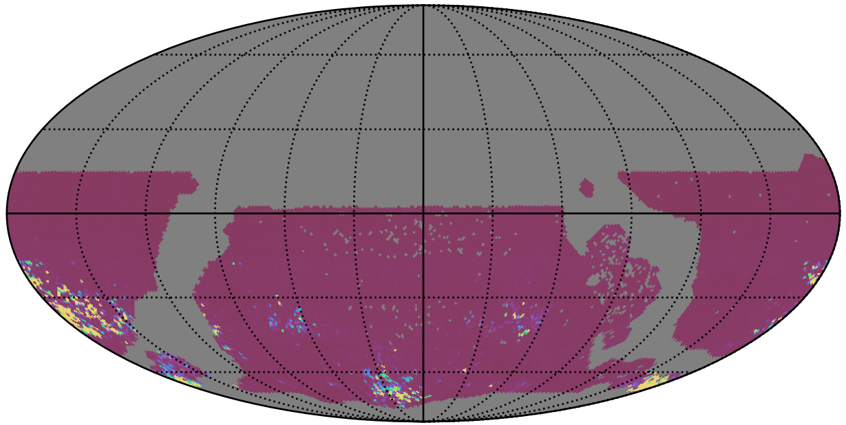
weather_cloudso0v3.4_10yrs WFD gr bands: 75th Percentile Intranight Timespan
