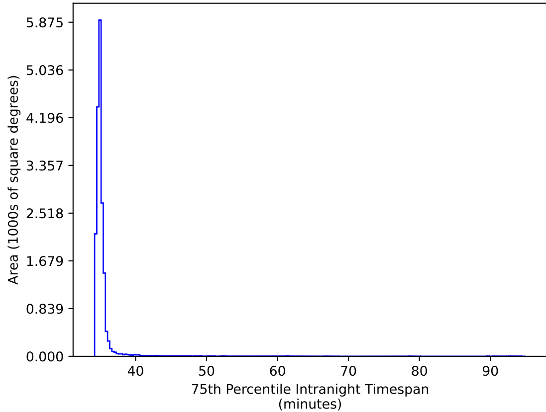
weather_cloudso0v3.4_10yrs WFD gr bands: 75th Percentile Intranight Timespan
