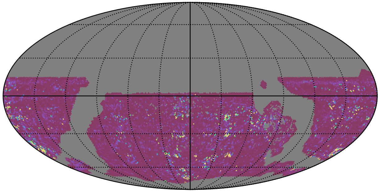
weather_cloudso0v3.4_10yrs WFD g band: 75th Percentile Intranight Timespan
