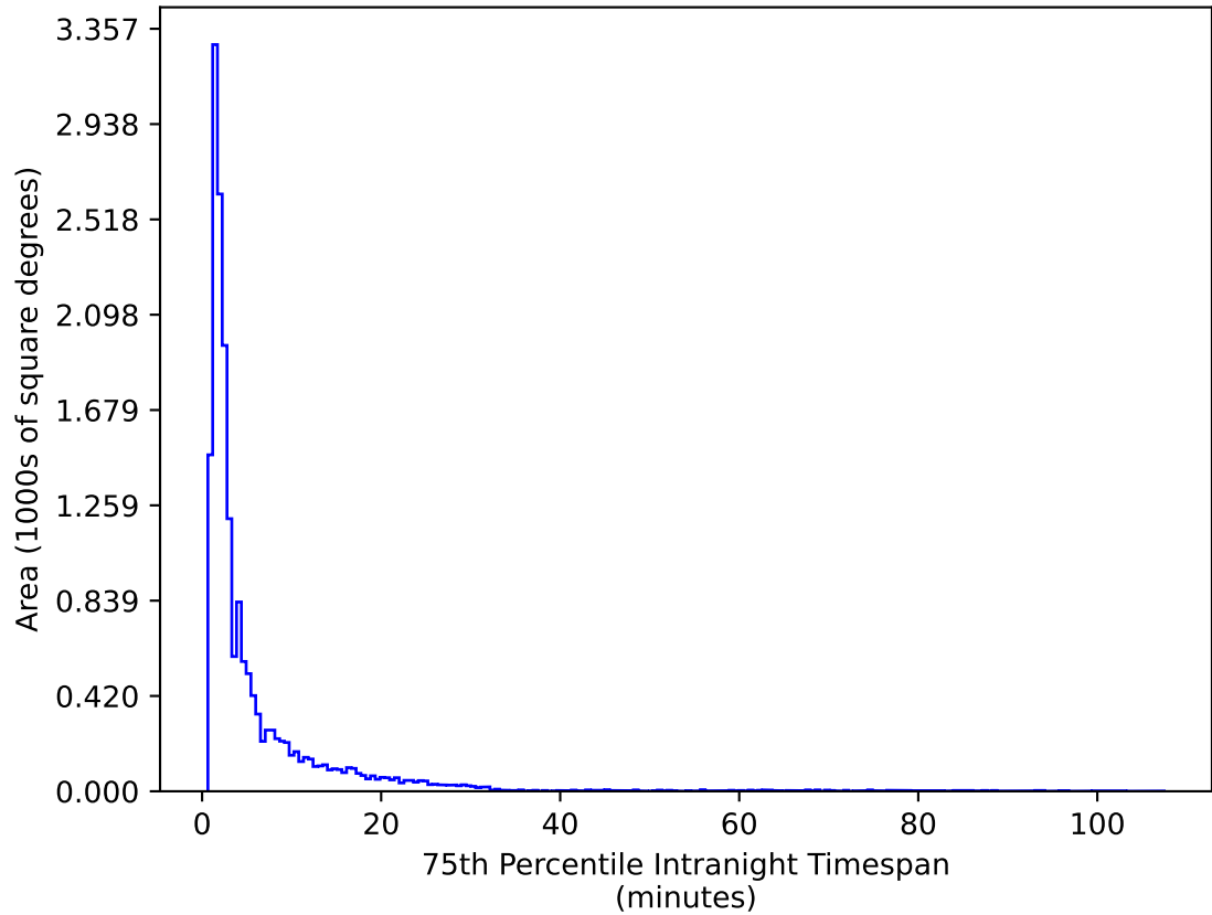
weather_cloudso0v3.4_10yrs WFD g band: 75th Percentile Intranight Timespan
