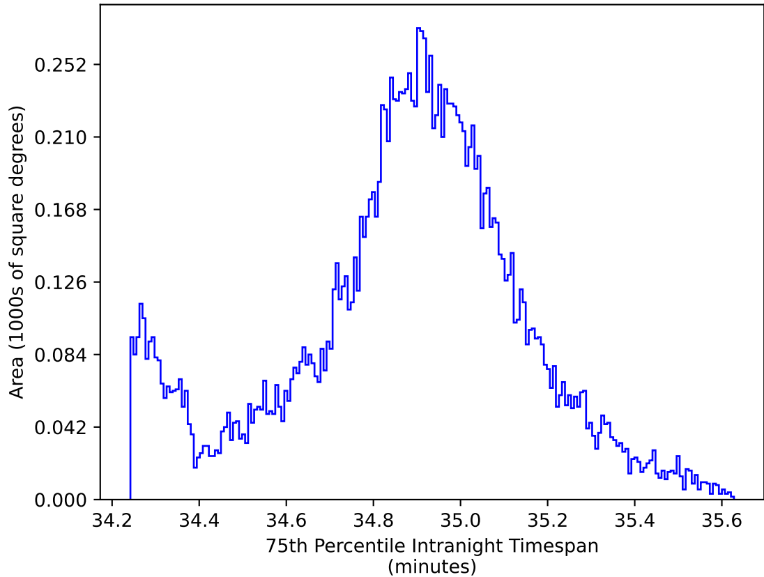
weather_cloudso0v3.4_10yrs WFD all bands: 75th Percentile Intranight Timespan
