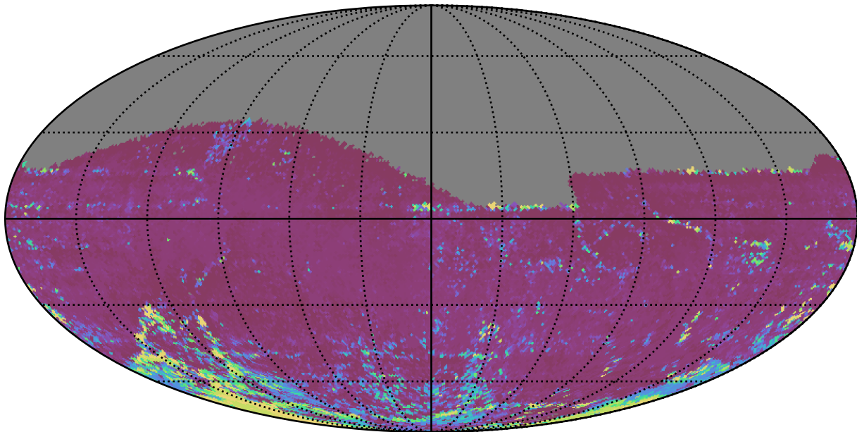
weather_cloudso0v3.4_10yrs All sky z band: 75th Percentile Intranight Timespan
