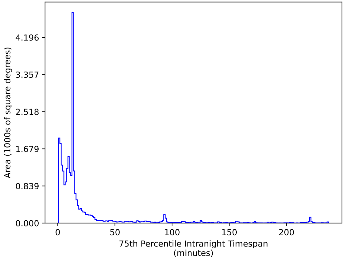
weather_cloudso0v3.4_10yrs All sky z band: 75th Percentile Intranight Timespan
