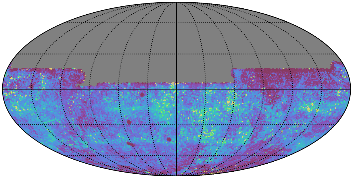
weather_cloudso0v3.4_10yrs All sky y band: 75th Percentile Intranight Timespan
