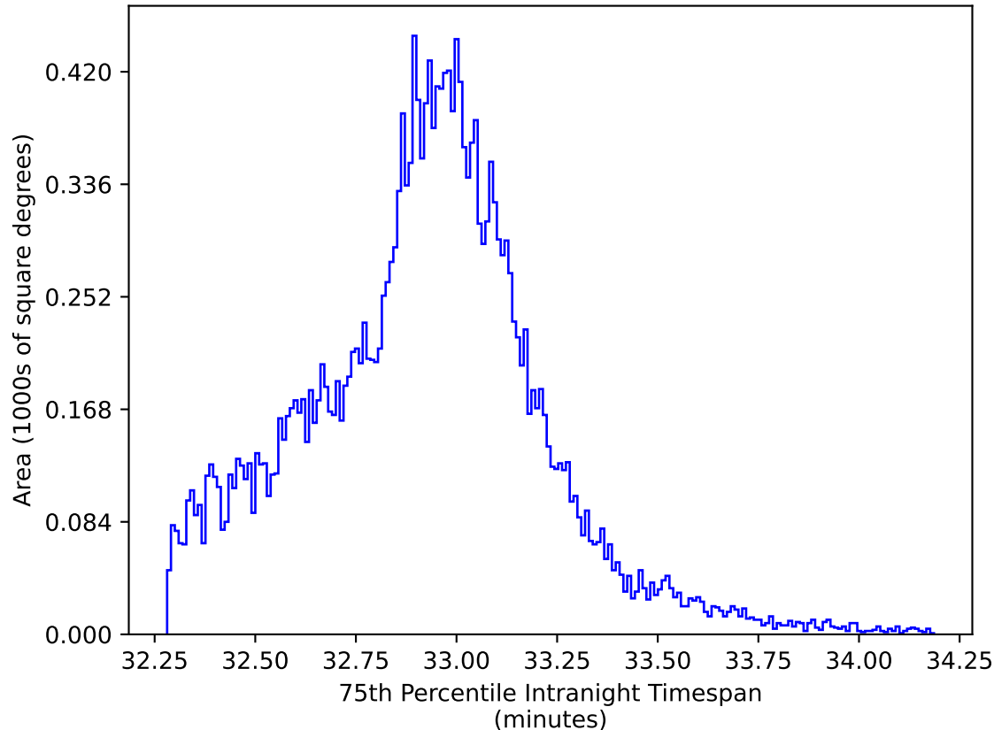
weather_cloudso0v3.4_10yrs All sky y band: 75th Percentile Intranight Timespan
