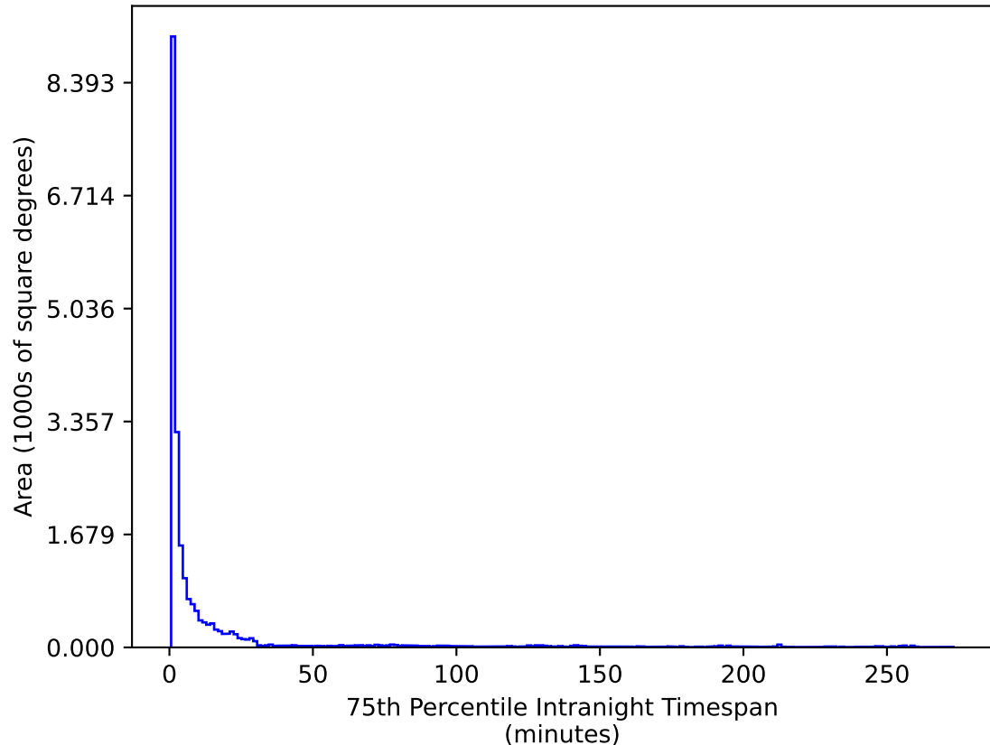
weather_cloudso0v3.4_10yrs All sky u band: 75th Percentile Intranight Timespan
