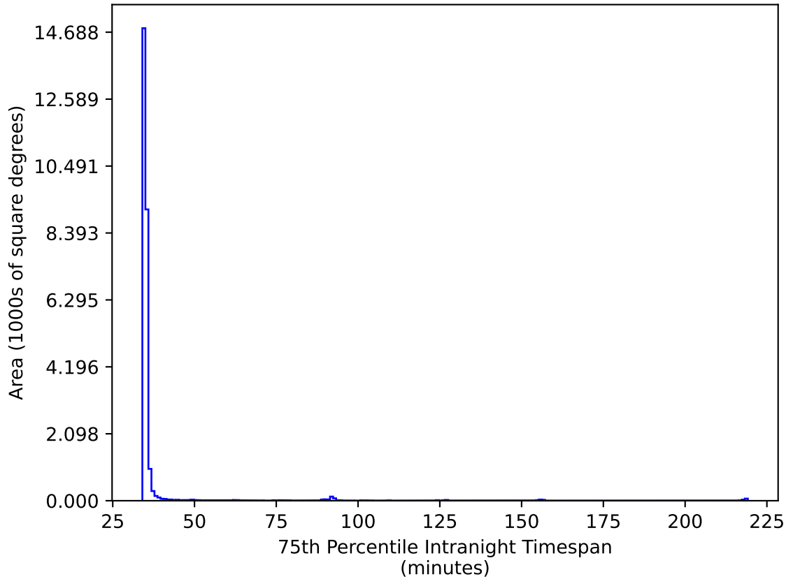
weather_cloudso0v3.4_10yrs All sky ri bands: 75th Percentile Intranight Timespan
