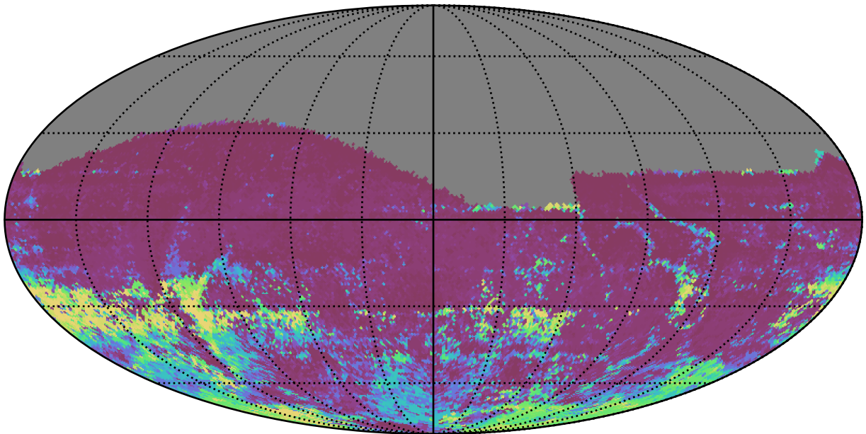
weather_cloudso0v3.4_10yrs All sky r band: 75th Percentile Intranight Timespan
