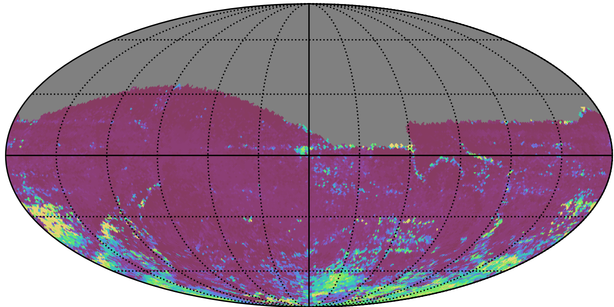
weather_cloudso0v3.4_10yrs All sky i band: 75th Percentile Intranight Timespan
