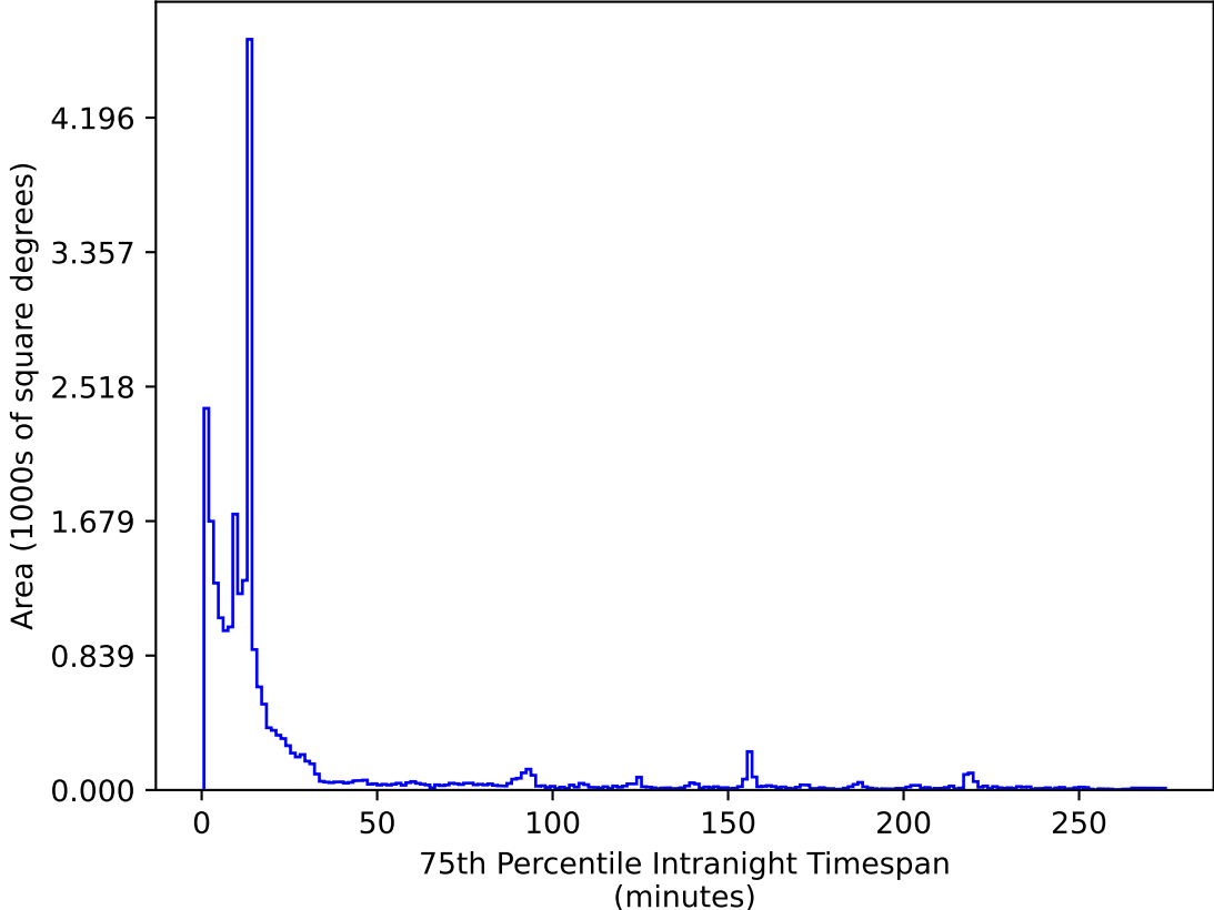
weather_cloudso0v3.4_10yrs All sky i band: 75th Percentile Intranight Timespan
