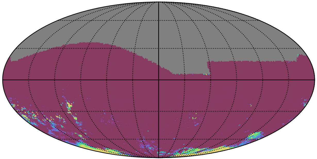
weather_cloudso0v3.4_10yrs All sky gr bands: 75th Percentile Intranight Timespan
